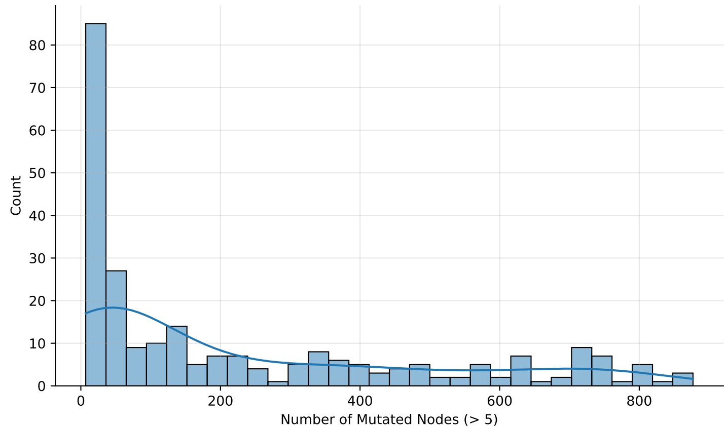
Transmission Rate 1_2 = 0.0005
