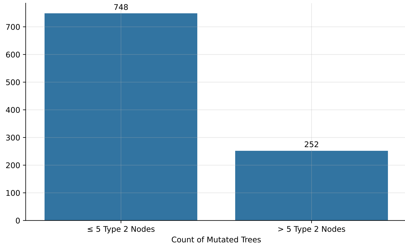
Transmission Rate 1_2 = 0.0005
