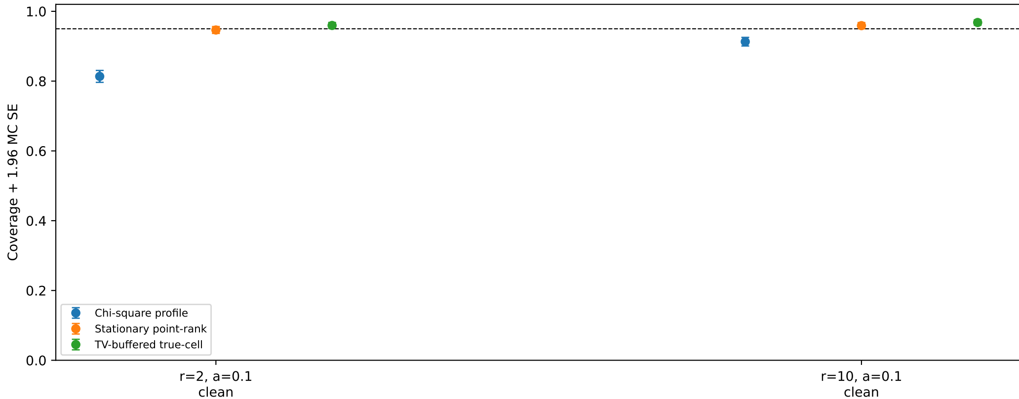
Finite-sample calibration: coverage and assumption stress
