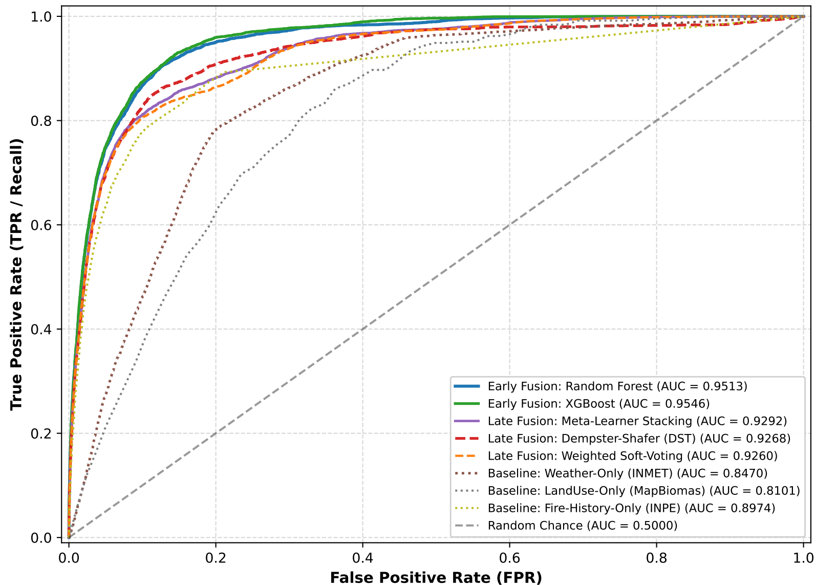
Receiver Operating Characteristic (ROC) on 2024-2025 Test Set
