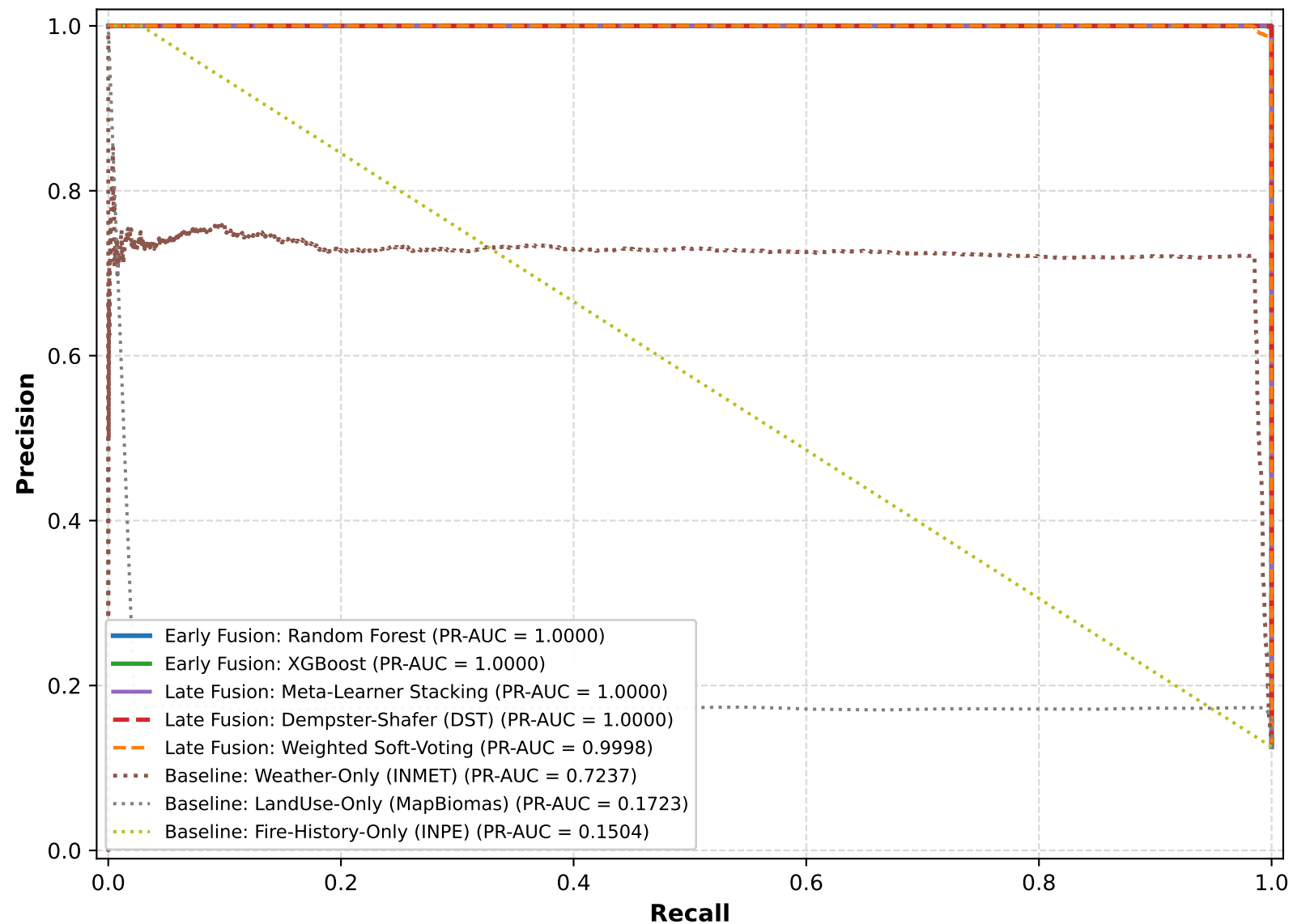
Precision-Recall Curves on Imbalanced 2024-2025 Test Set
