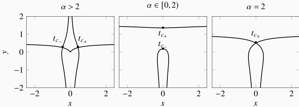
Figure 2 – The lines represent the solution to \text{Im}[f(z) - f(t_c)] = 0 for the three possible cases of the Hermite Polynomial. These are the curves we use to perform the asymptotic analysis on the integral. Note the case \alpha = 2 ; the coalescence of critical point gives origin to the Airy function.
