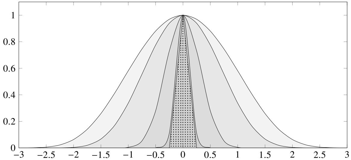
Figure 1 – In the Plot it is represented the plot for e^{-\lambda(\cosh(x)-1)} and an increasing \lambda = 1, 2, 10, 70 - darker represent larger values of the parameter. The dotted patten represents e^{-\lambda x^2} for large lambda.
