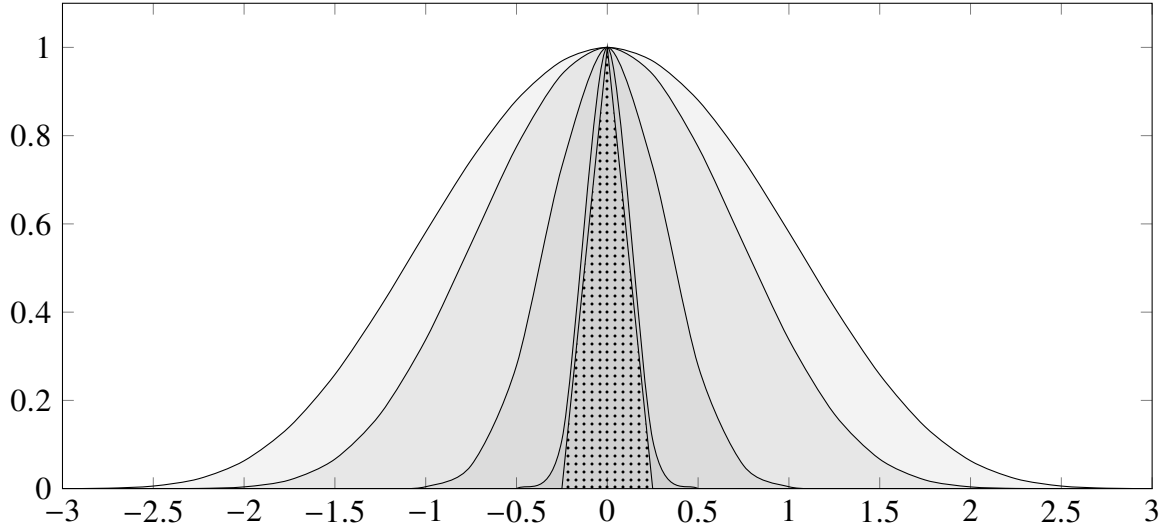
Figure 12 – In the Plot it is represented the plot for e^{-\lambda(\cosh(x)-1)} and an increasing \lambda = 1, 2, 10, 70 - darker represent larger values of the parameter. The dotted patten represents e^{-\lambda x^2} for large lambda.
