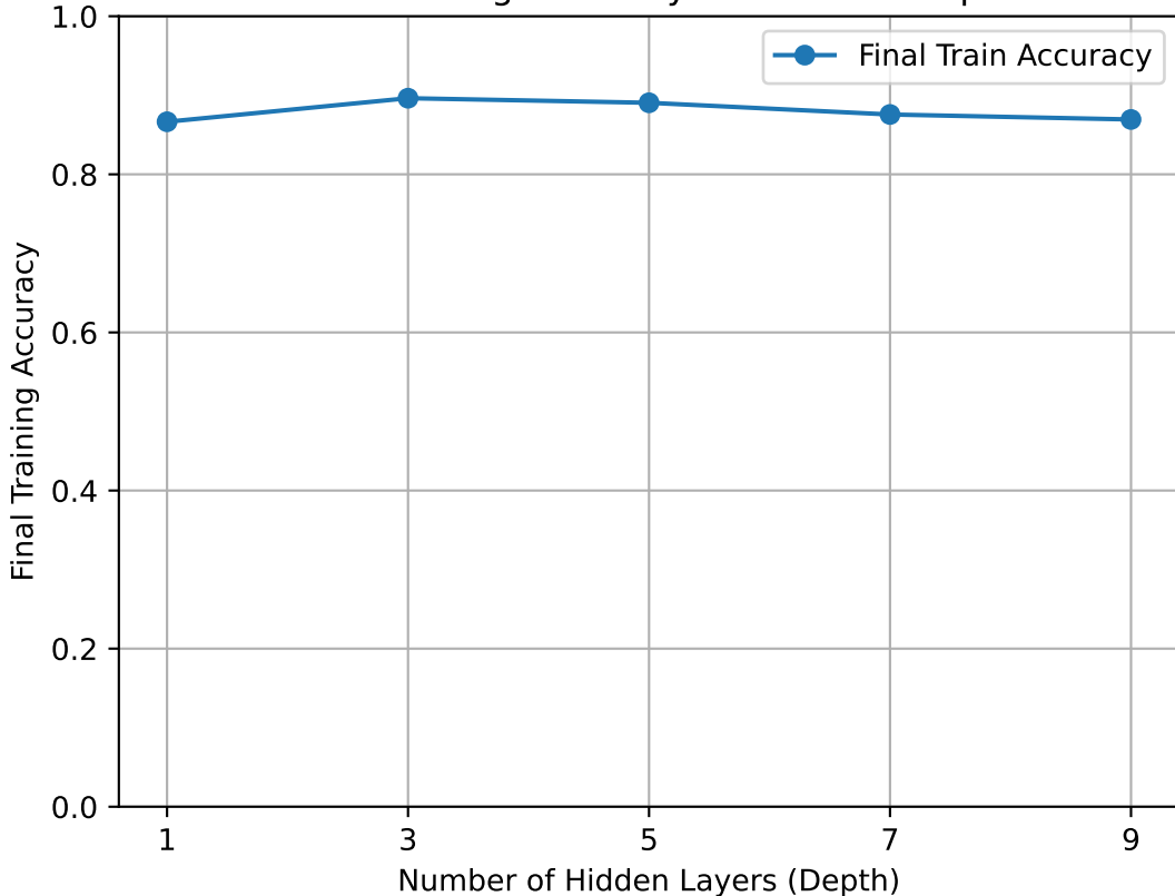
Final Training Accuracy vs Network Depth
