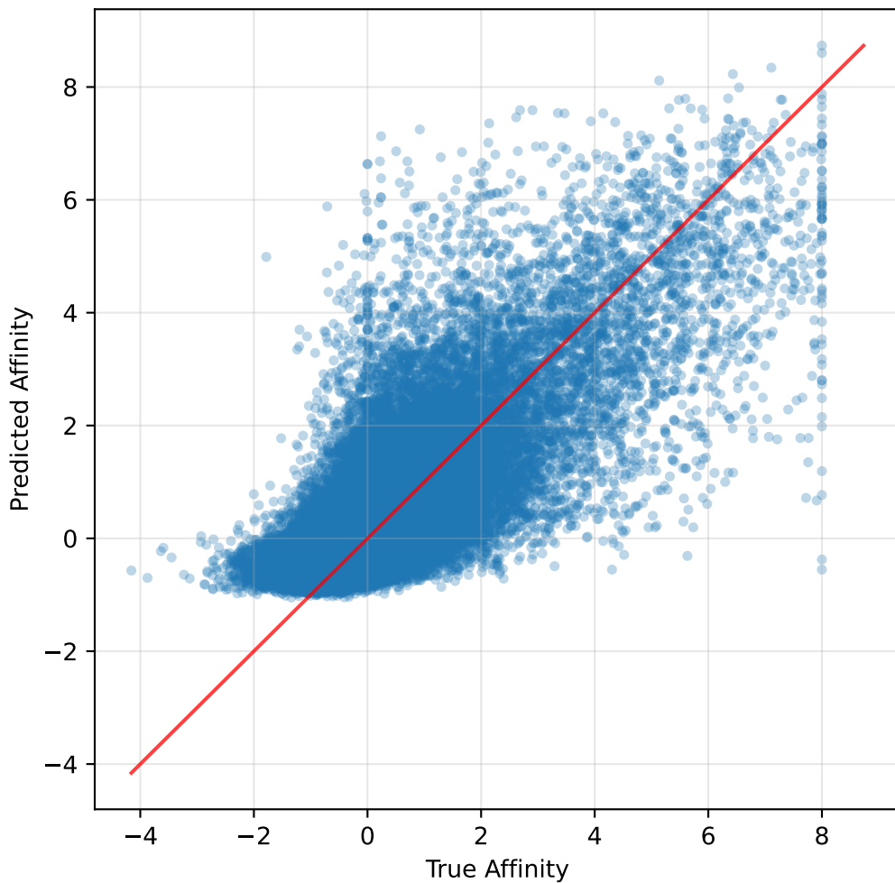
TransformerEncoder: True vs Predicted
