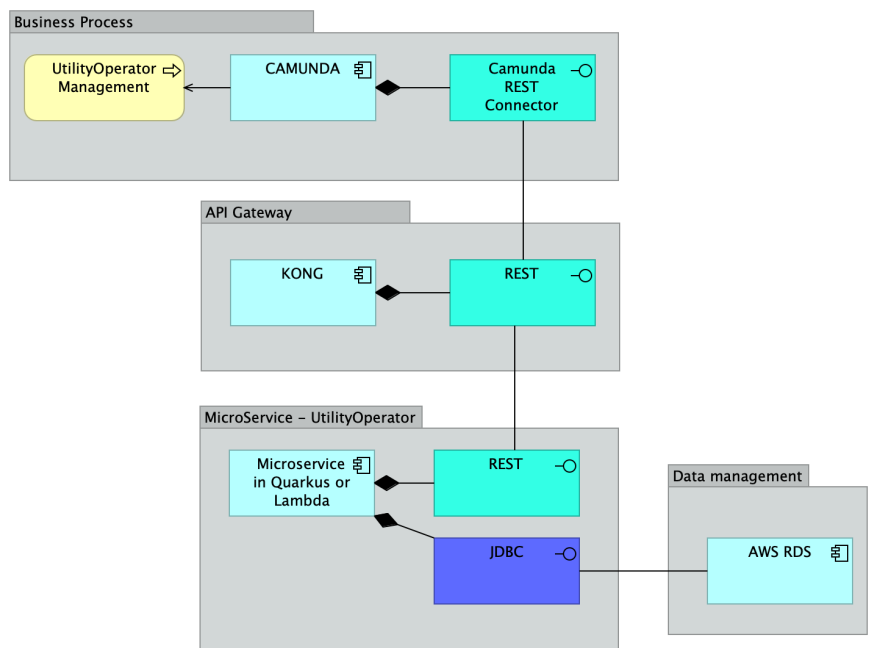
Figure 5. The integration architecture of Utility Operator microservice.
