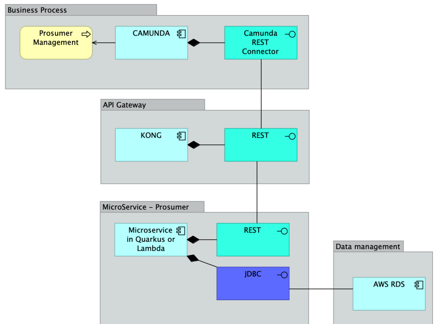
Figure 4. The integration architecture of Prosumer microservice.
