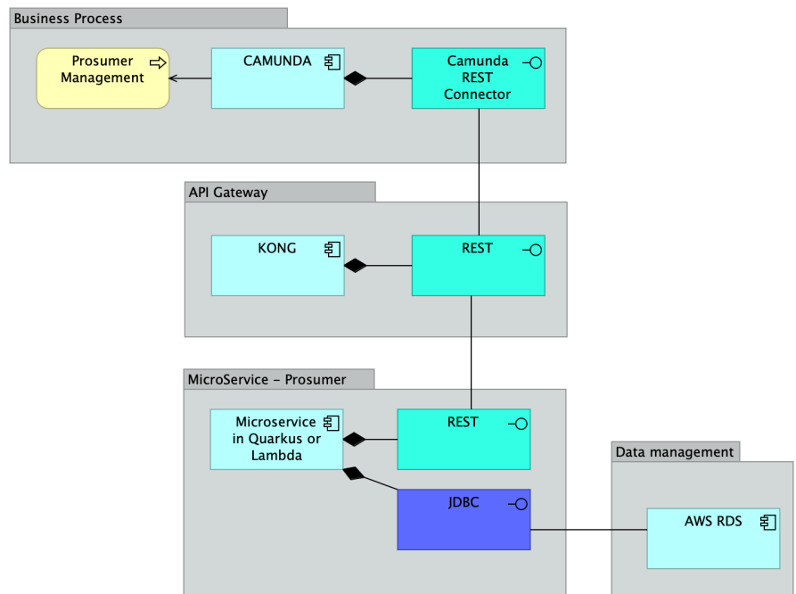
Figure 4. The integration architecture of Prosumer microservice.
