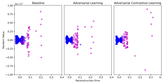
Fig. 6. The visualization of reconstruction errors for test set samples obtained using various learning strategies on Dataset B. The magenta dots indicate anomaly samples, while the blue dots represent normal samples. The horizontal axis signifies the reconstruction error, while the vertical axis is associated with random values to enable a two-dimensional visualization of the reconstruction error.
