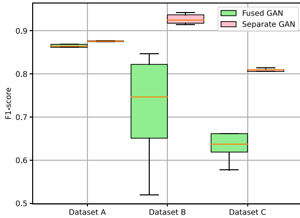
Fig. 4. The comparison between Fused GAN and Separate GAN (i.e., Method 6 in Table III) with 10 times running. The discriminator of Fused GAN utilizes two 1D CNNs to embed data from the log and metric modalities separately. These embeddings are then fused using MSA to obtain a unified representation, which is finally used by the classification layer to discriminate whether the input data is real or reconstructed.
