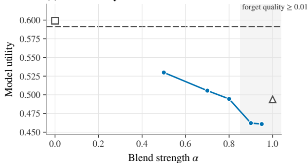
(c) Model utility
