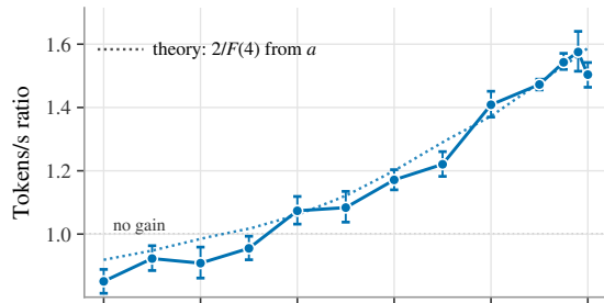
(b) Speed-up, k = 4 over k = 1
