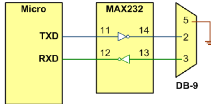
(b) MAX232 Connection to the Microcontroller / Microprocessor
