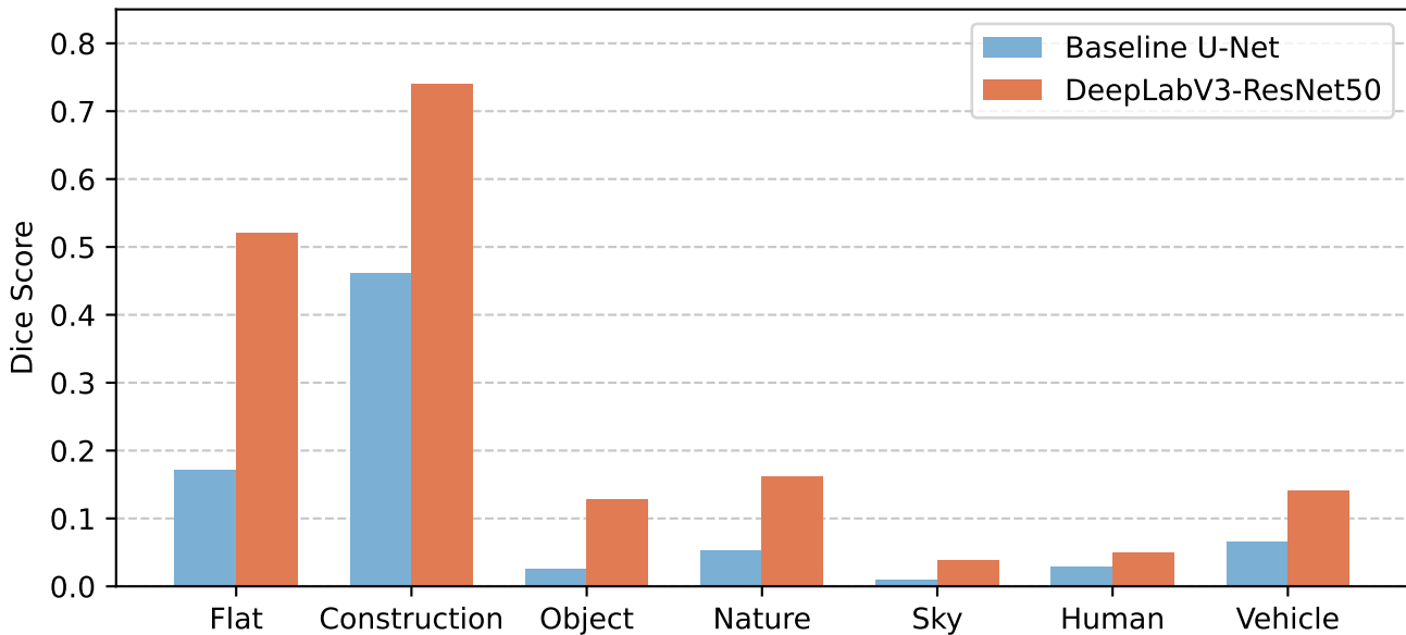
Per-Category Dice Scores under Corruptions
