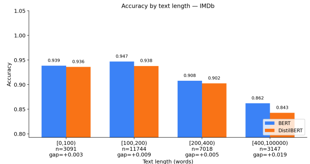
(b) IMDb: the teacher–student gap grows with review length, consistent with long-context integration as a failure mode.
