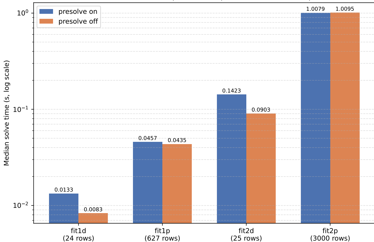
Solve time: real Netlib primal/dual pairs (HiGHS dual simplex)
