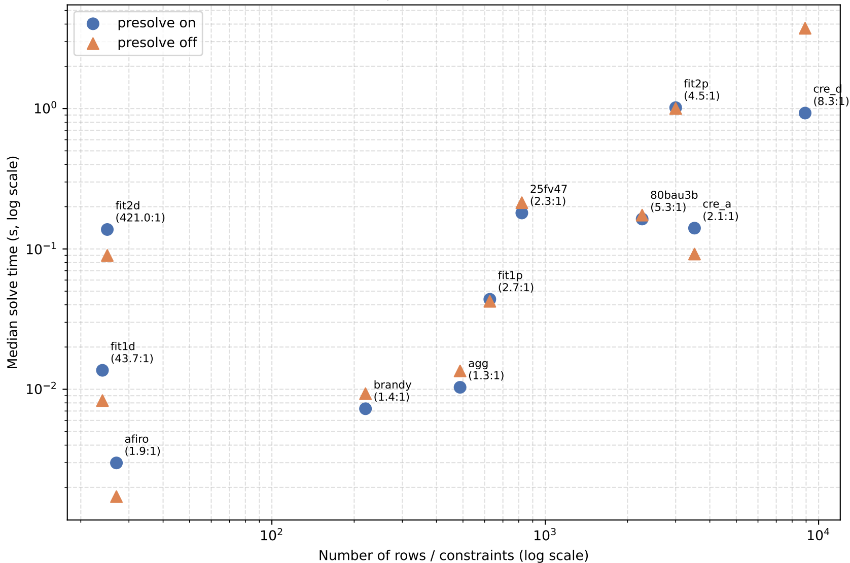
Solve time vs. row count across real Netlib LP instances (HiGHS dual simplex; labels show cols:rows ratio)
