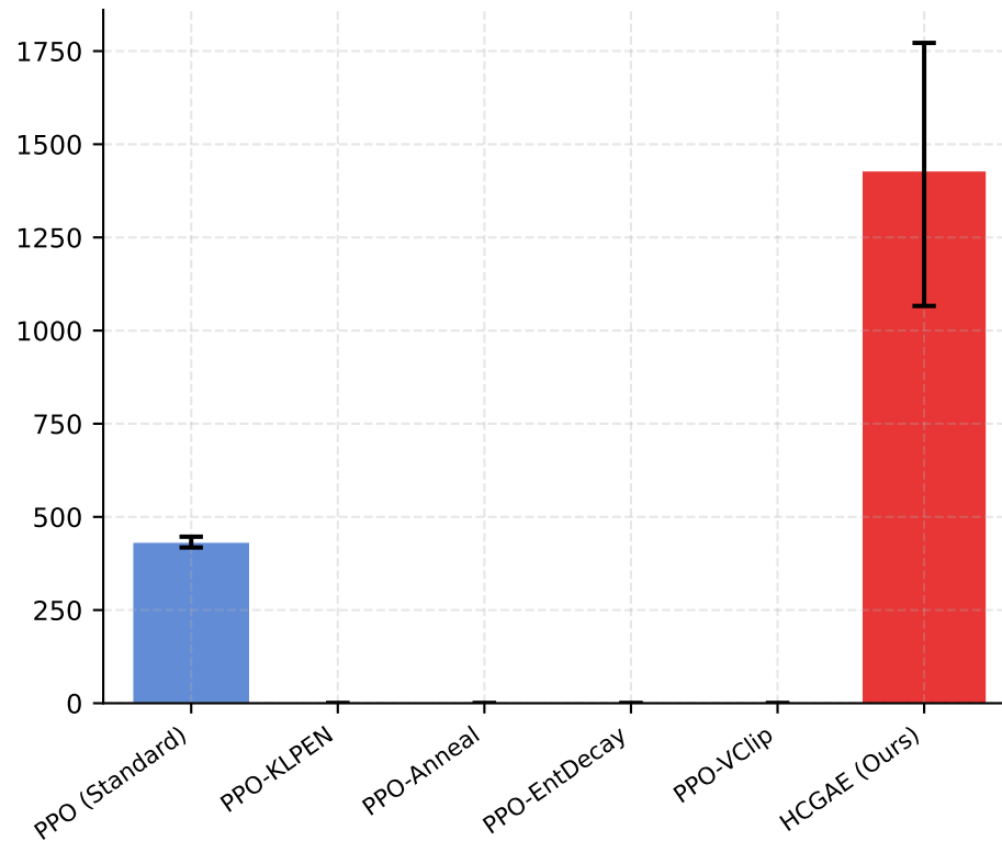
Walker2d-v4
