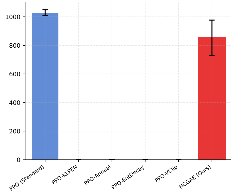
HalfCheetah-v4
