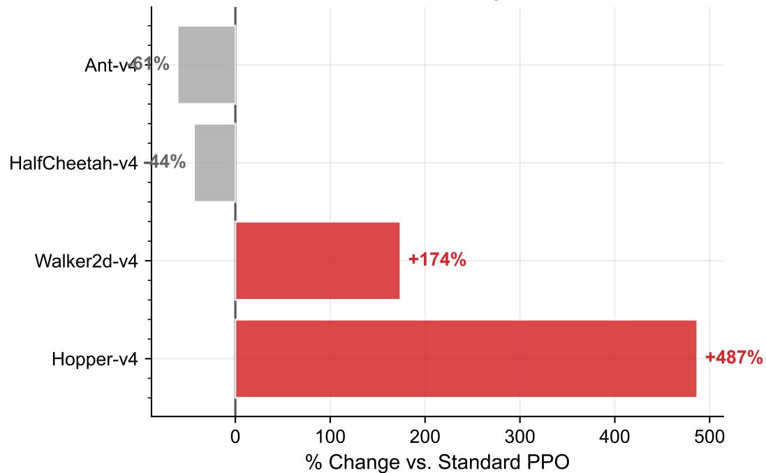
DCPPO-S Relative Improvement
