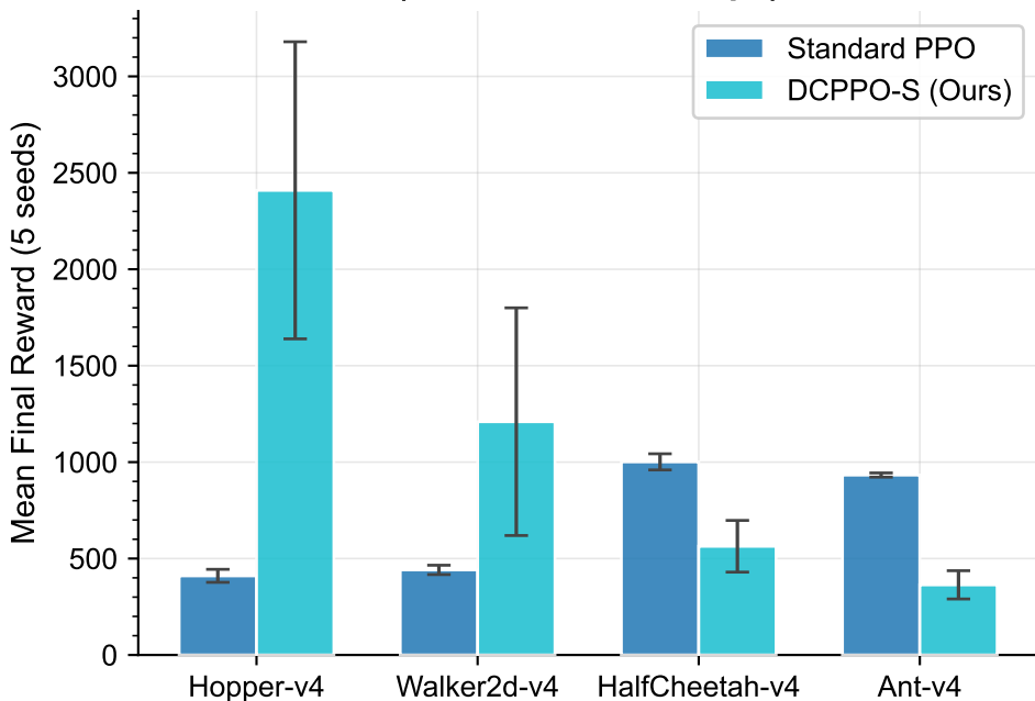
DCPPO-S vs. Standard PPO (5 Seeds × 300K Steps)
