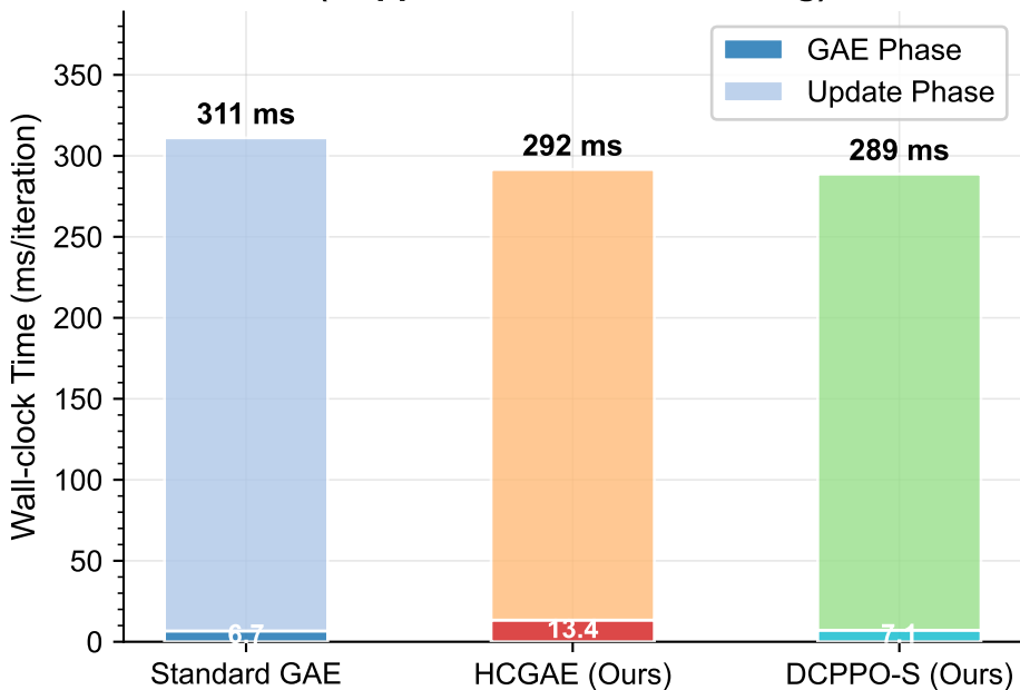
Per-Iteration Wall-Clock Time (Hopper-v4, CPU, 20 runs avg)
