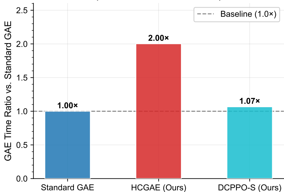
GAE Computation Overhead (Relative to Standard GAE)
