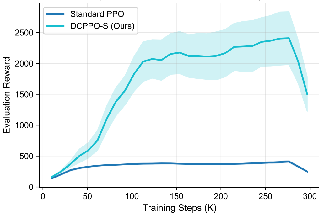
DCPPO-S vs. Standard PPO (Hopper-v4, 5 Seeds, Mean \pm SEM)
