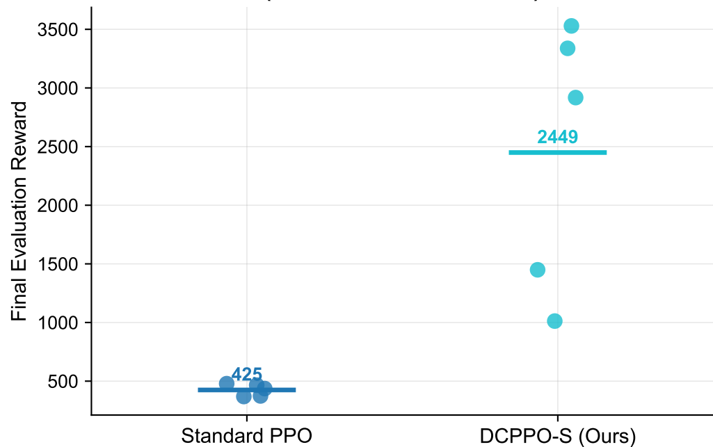
Per-Seed Final Rewards (Lines show 5-seed mean)
