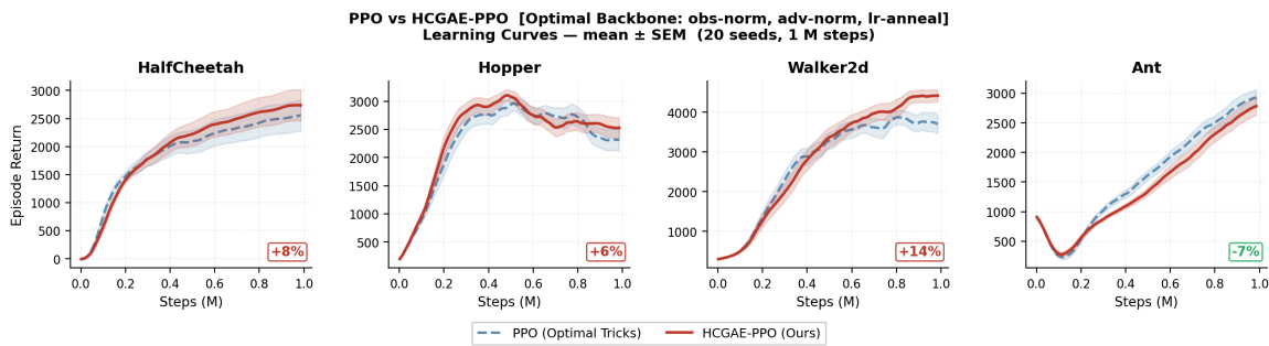
Figure 1: PPO learning curves OptimalBackbone
