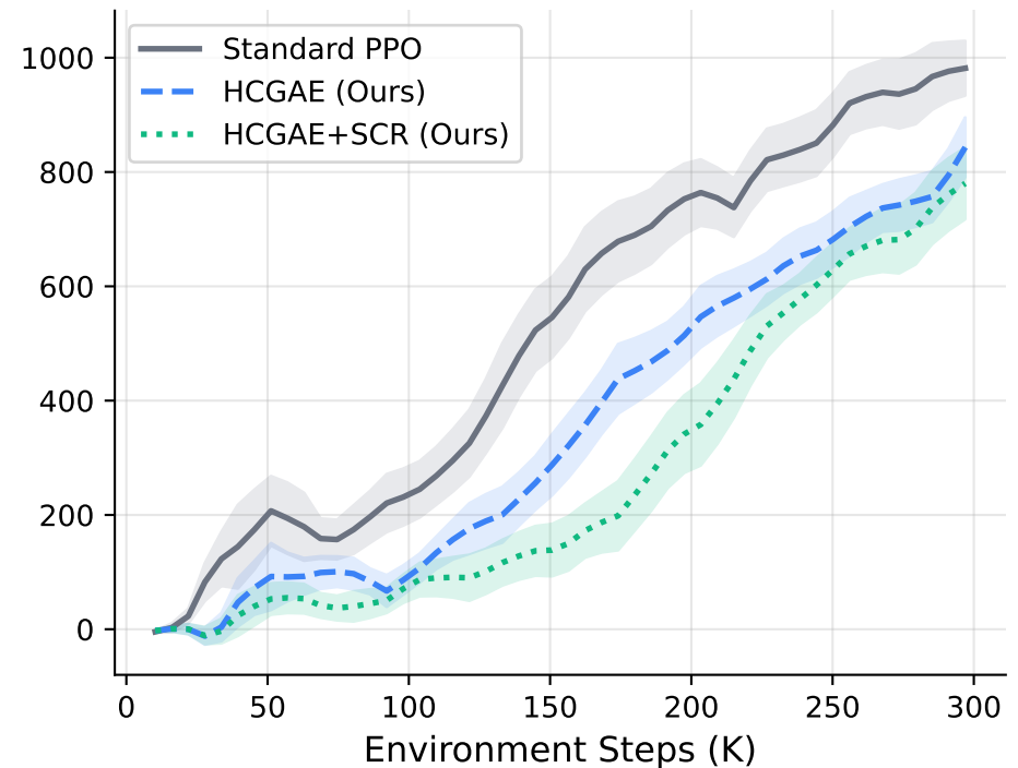
HalfCheetah-v4
