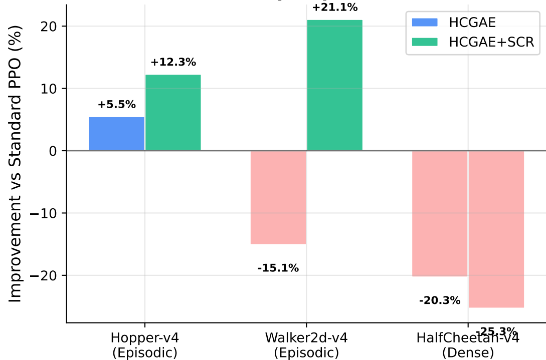
Environment-Dependent Performance (n=10 seeds, 300K steps; *p<0.05 on HalfCheetah)
