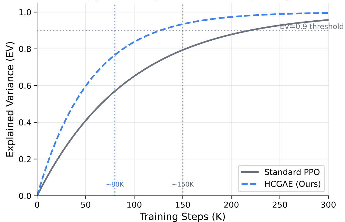
Critic Convergence: HCGAE vs Standard PPO (Hopper-v4, representative trajectory)
