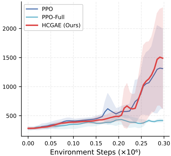
Walker2d-v4
