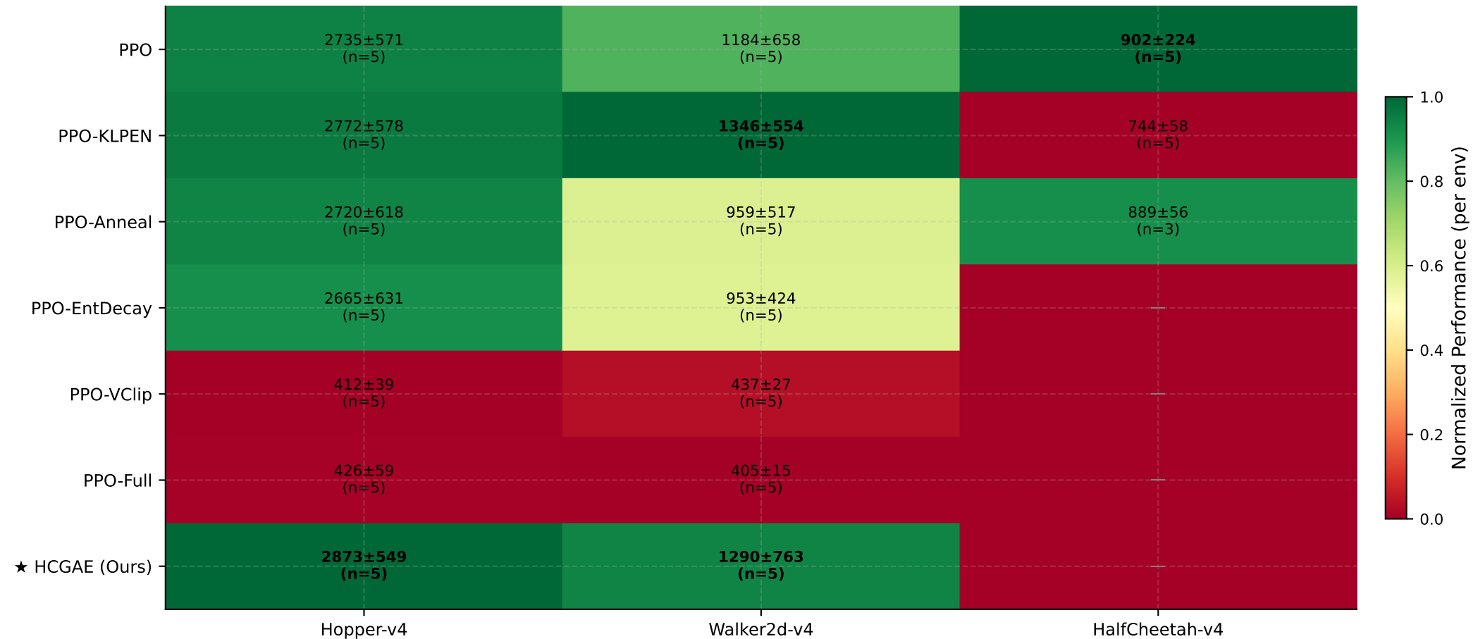
Final Performance: Mean \pm Std (5 seeds, last 5 evals) Color: relative rank within environment (green=best, red=worst)
