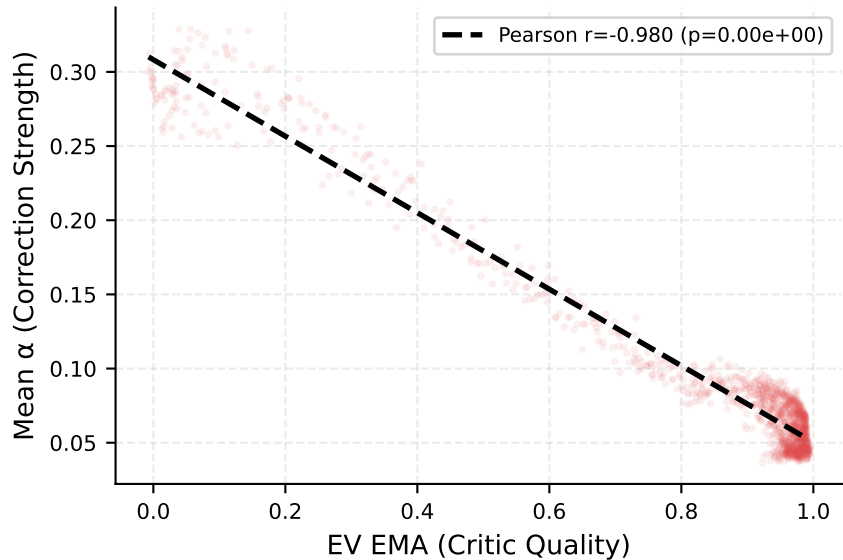
EV vs \alpha : Higher Critic Quality \rightarrow Smaller Correction (Design Verification)
