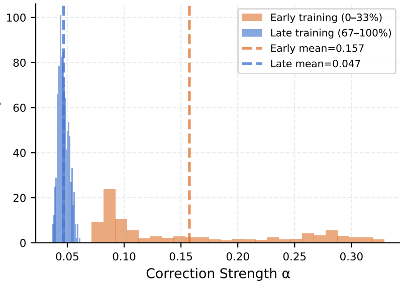
\alpha Distribution: Early vs Late Training (Hopper + Walker2d)
