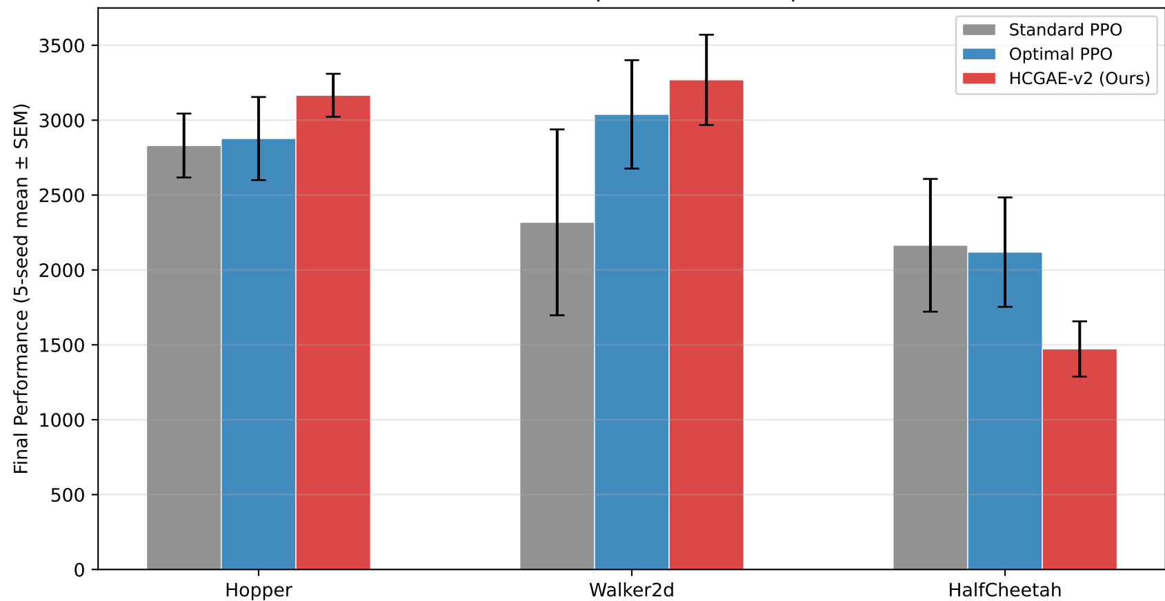
Final Performance Comparison (500K steps, 5 seeds)
