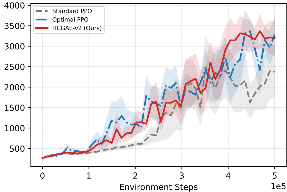
Walker2d
