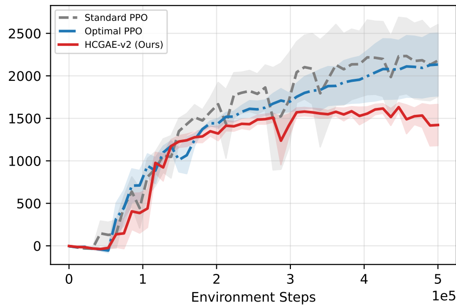
HalfCheetah
