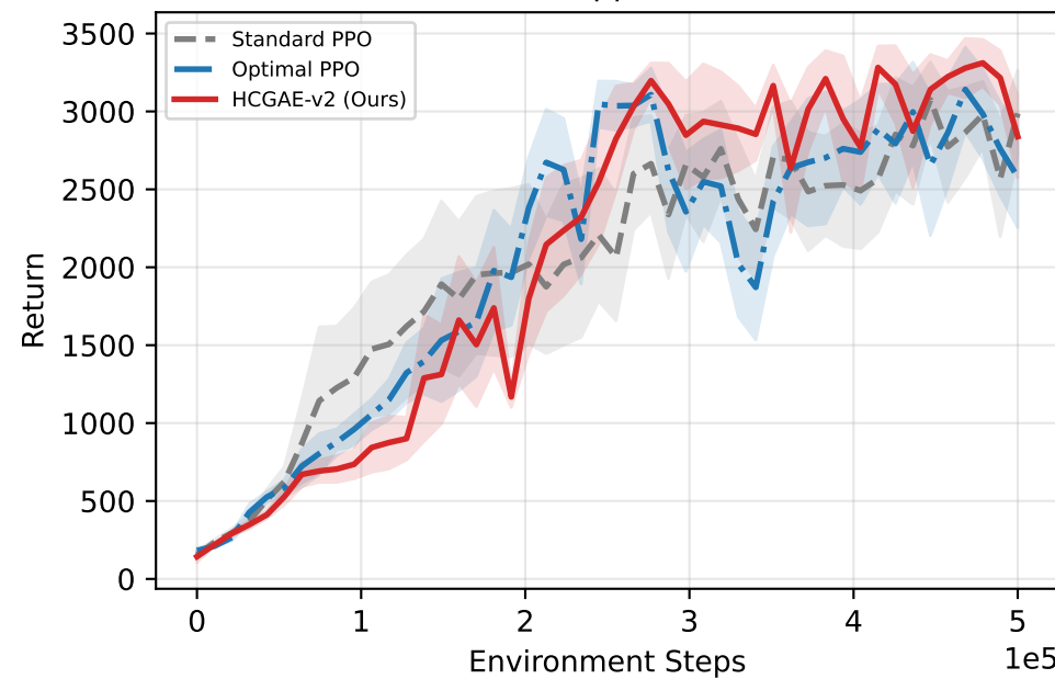
Hopper
