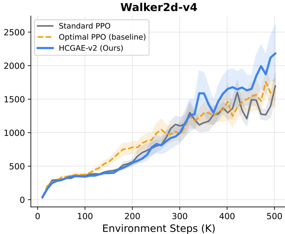
Learning Curves: HCGAE-v2 vs. Optimal PPO Baseline (n=5 seeds, 500K steps)
