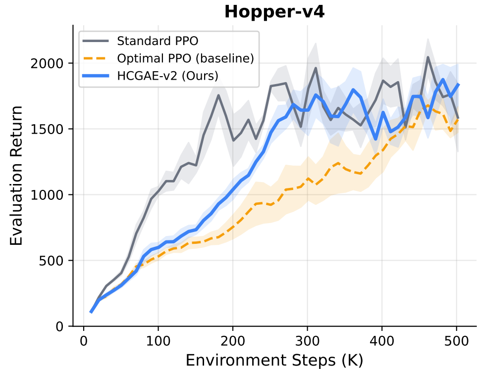
Learning Curves: HCGAE-v2 vs. Optimal PPO Baseline (n=5 seeds, 500K steps)
