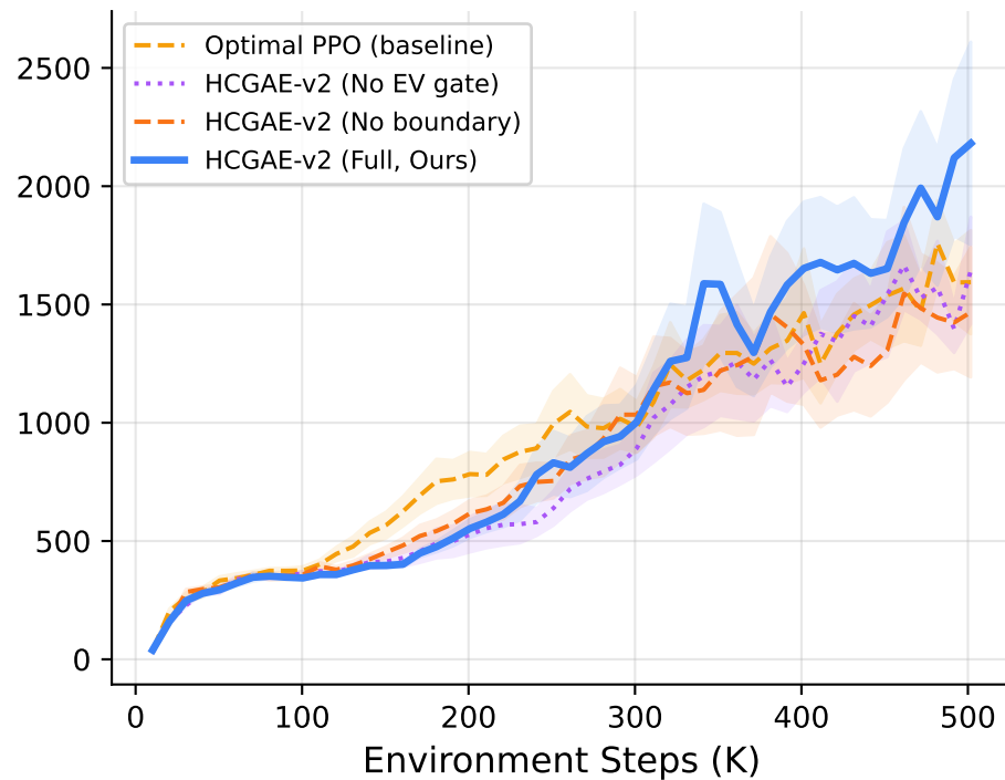
Walker2d-v4
