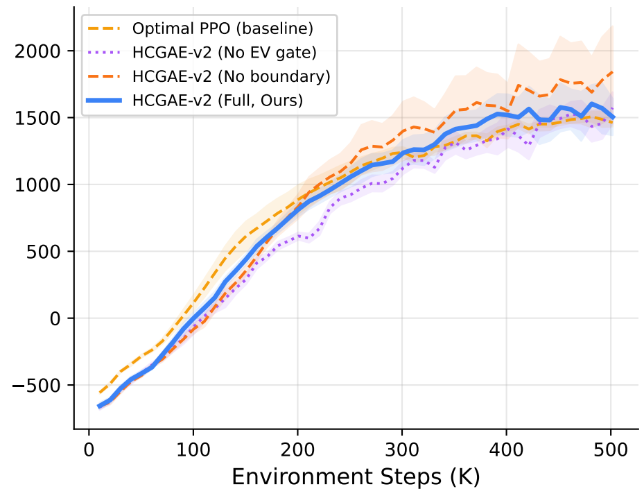
HalfCheetah-v4
