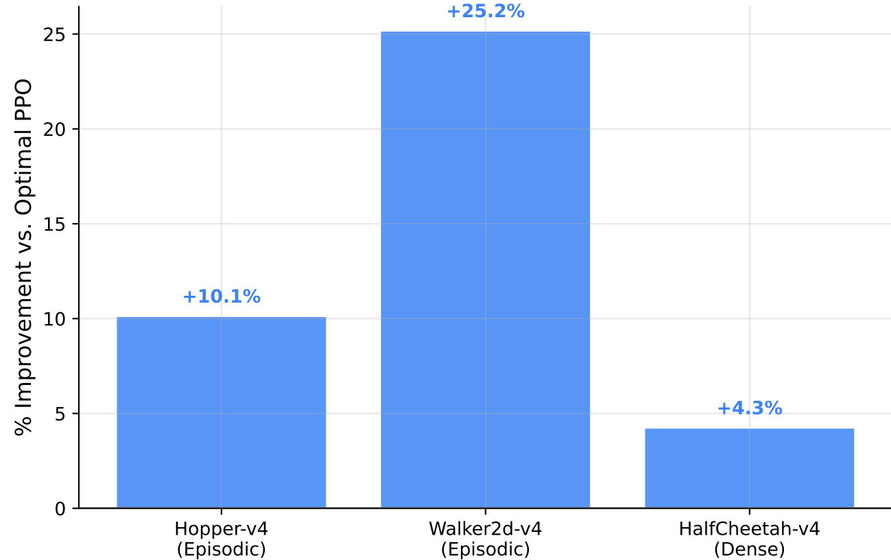
HCGAE-v2 Advantage per Environment (+: HCGAE-v2 better; -: HCGAE-v2 worse)
