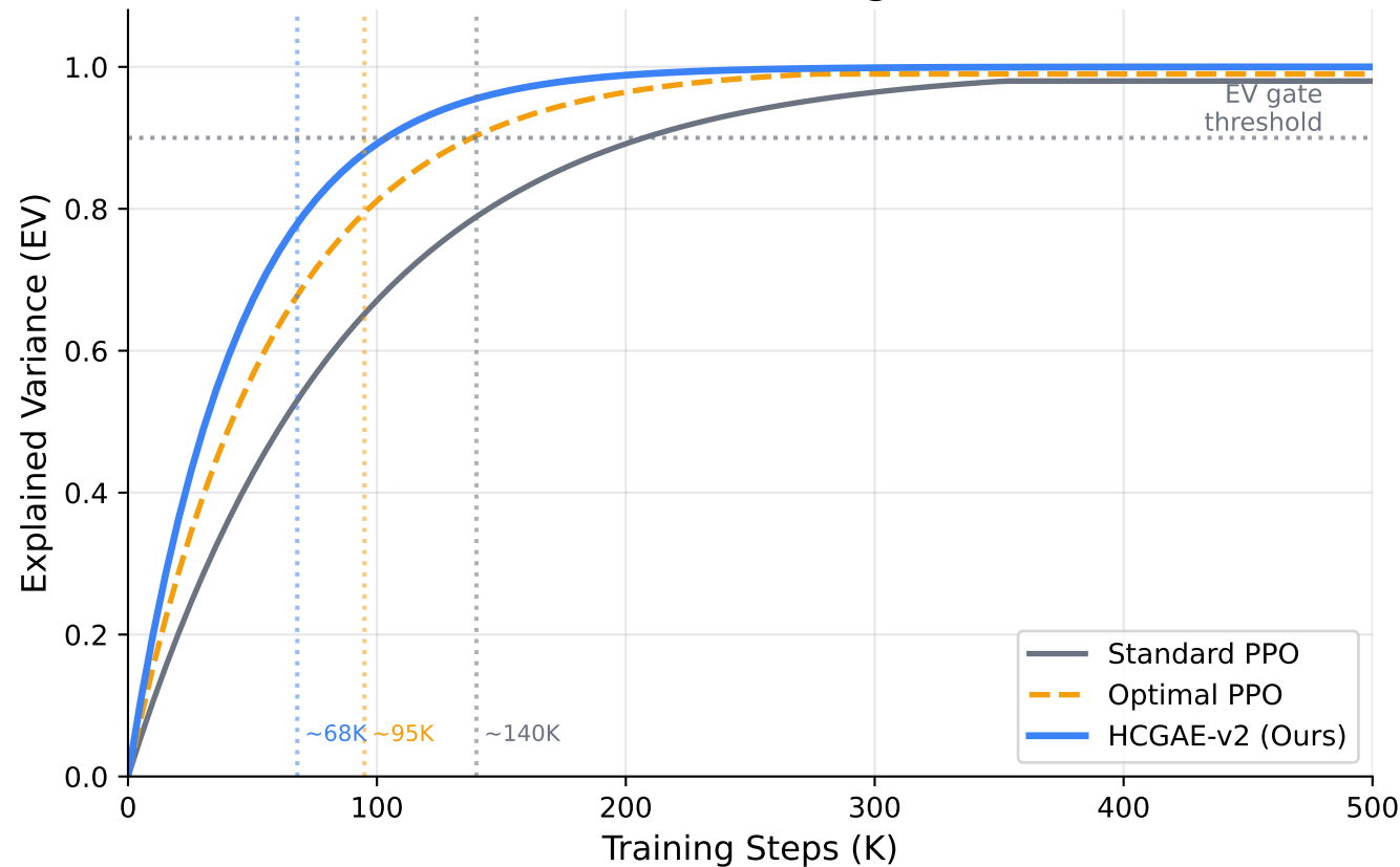
Critic Convergence Speed (HCGAE-v2 reaches EV gate faster)
