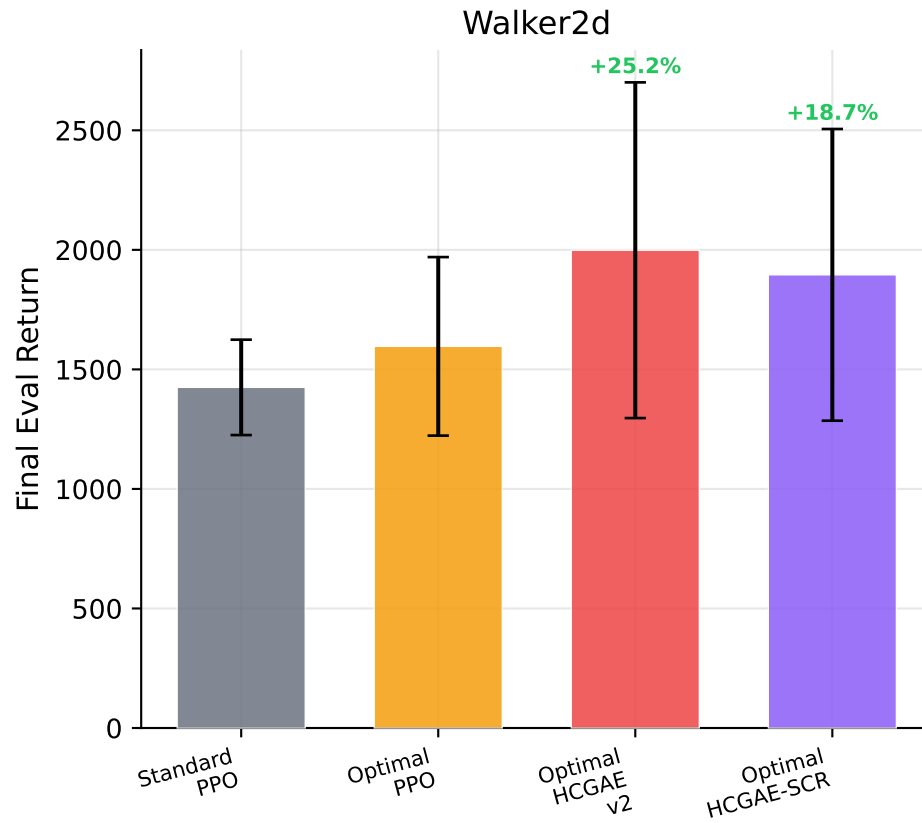
Final Performance: Optimal PPO Baseline (5 seeds, 500K steps)
