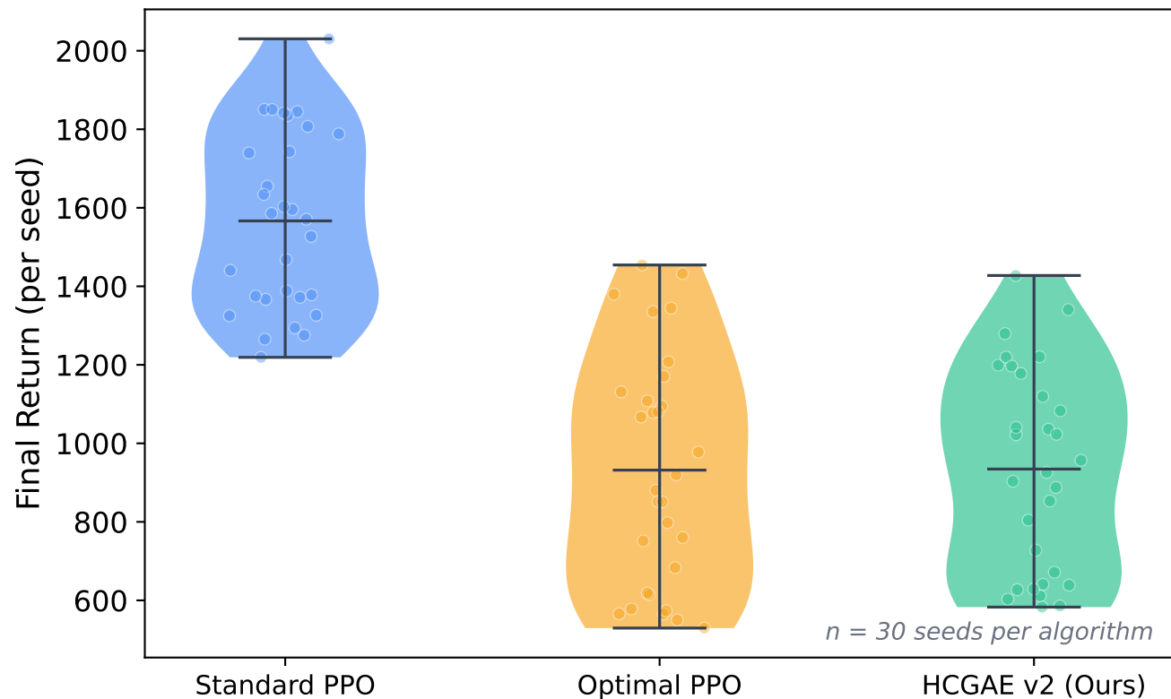
(b) Distribution of Individual Seeds
