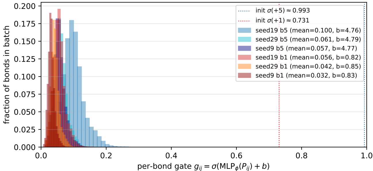
V2-T5 trained per-bond gate distribution on BACE (b=+5 vs b=+1 init)
