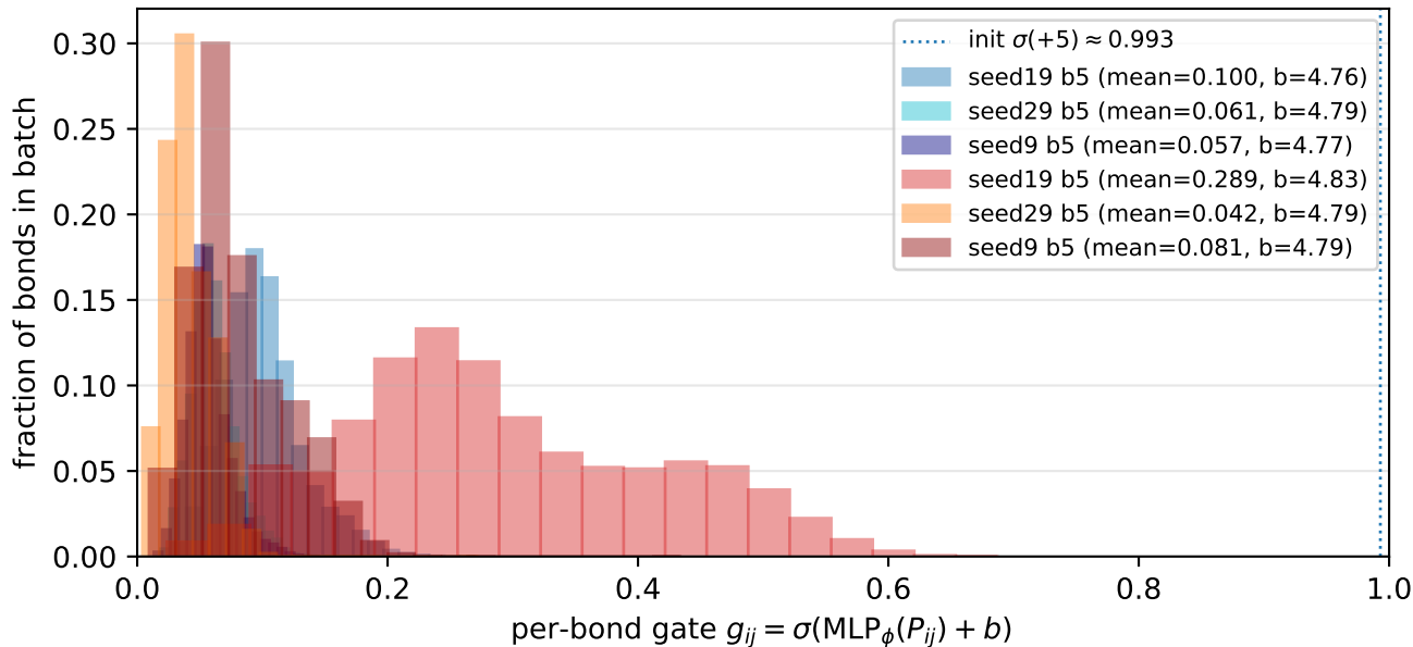
V2-T5 trained gate distribution: BACE (FP-saturated) vs BBBP (V2 wins)
