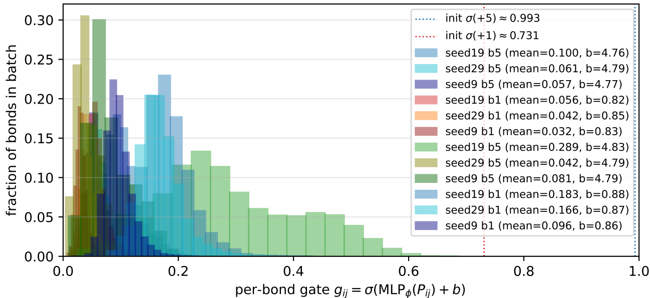
V2-T5 trained gates: 2 datasets x 2 bias inits x 3 seeds
