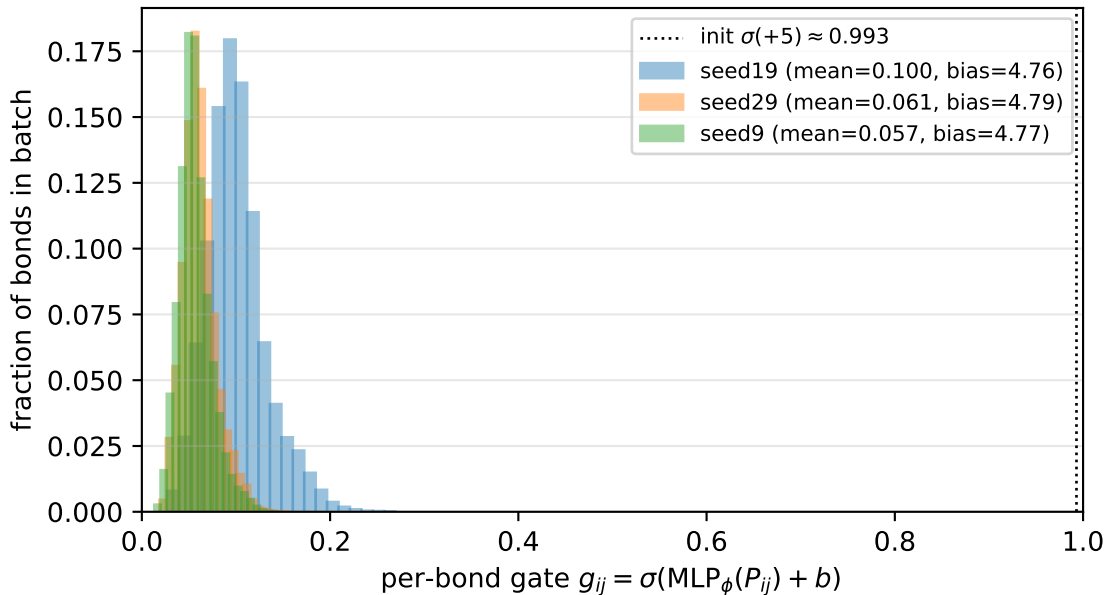
V2-T5 trained per-bond gate distribution on BACE (b=+5 init)
