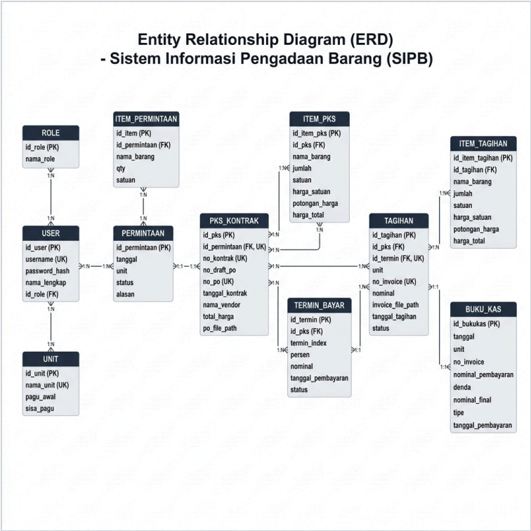
Gambar 1.3 Entity Relationship Diagram (ERD) Normalisasi Level 3
