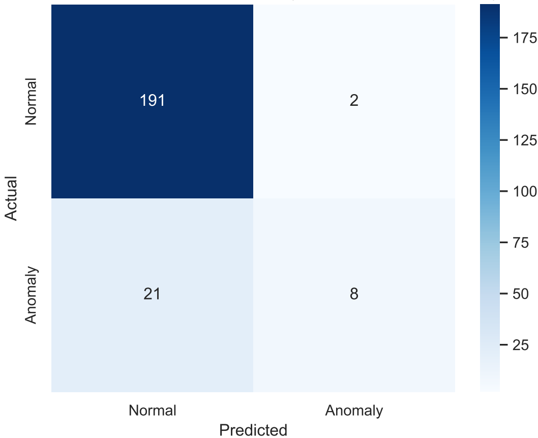
Confusion Matrix - LSTM autoencoder (bidirectional + Mahalanobis)
