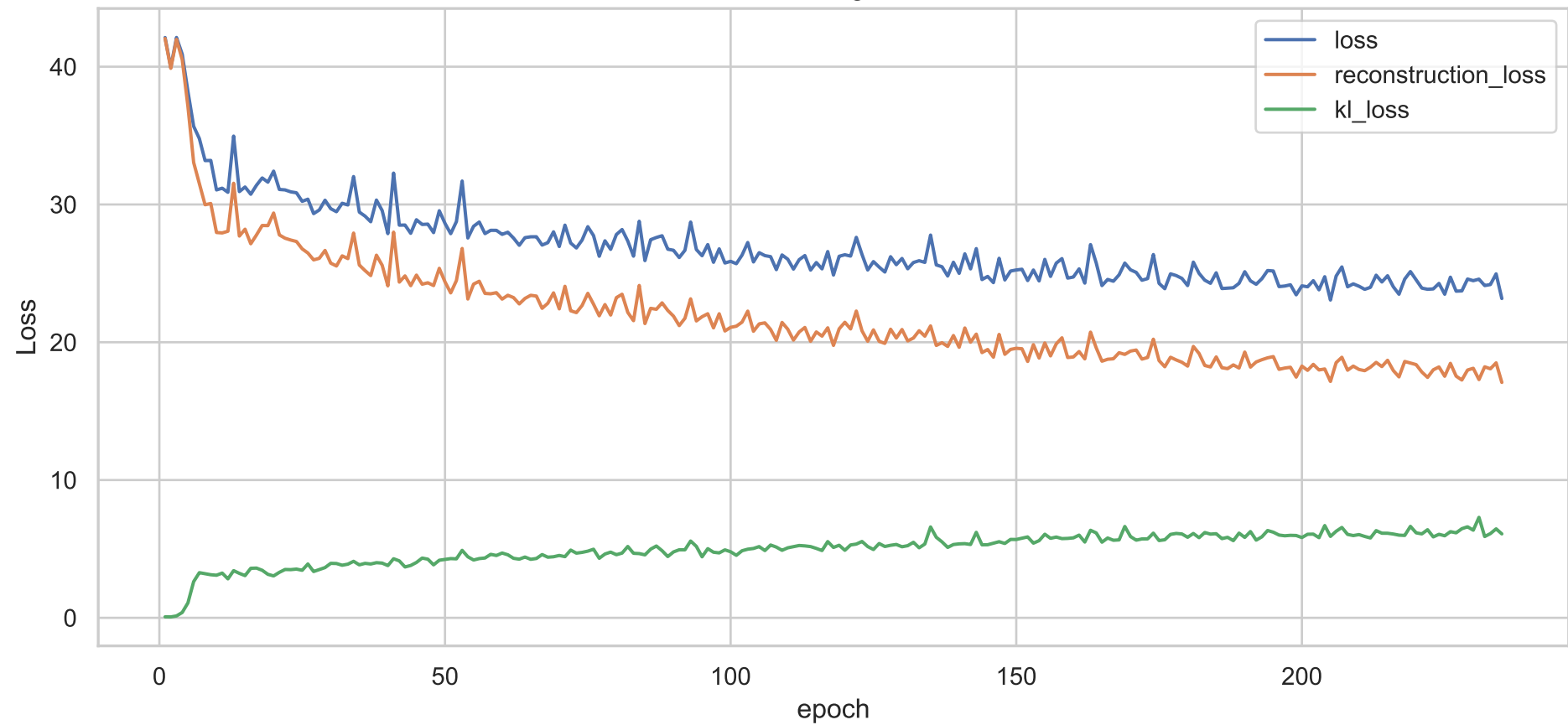
VAE training losses
