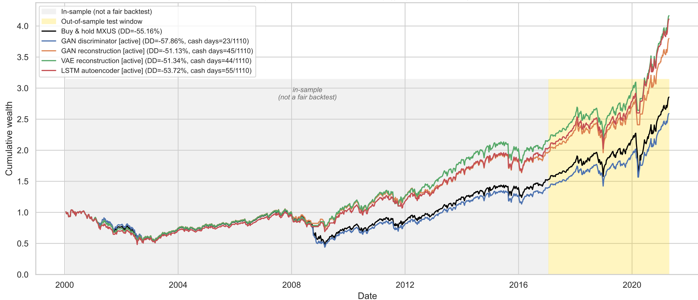
Risk-managed equity curve over full MXUS history (gray = in-sample, gold = out-of-sample)
