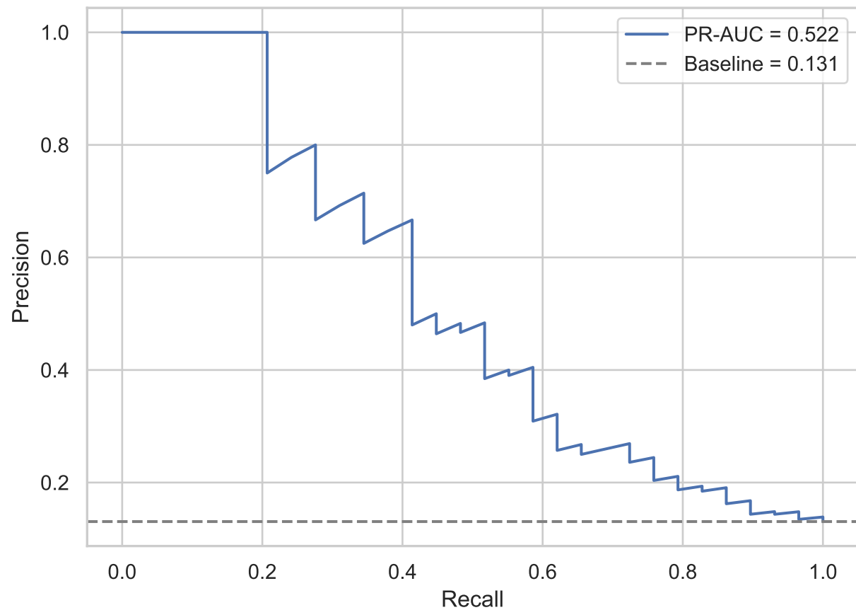
Precision-Recall - VAE reconstruction score
