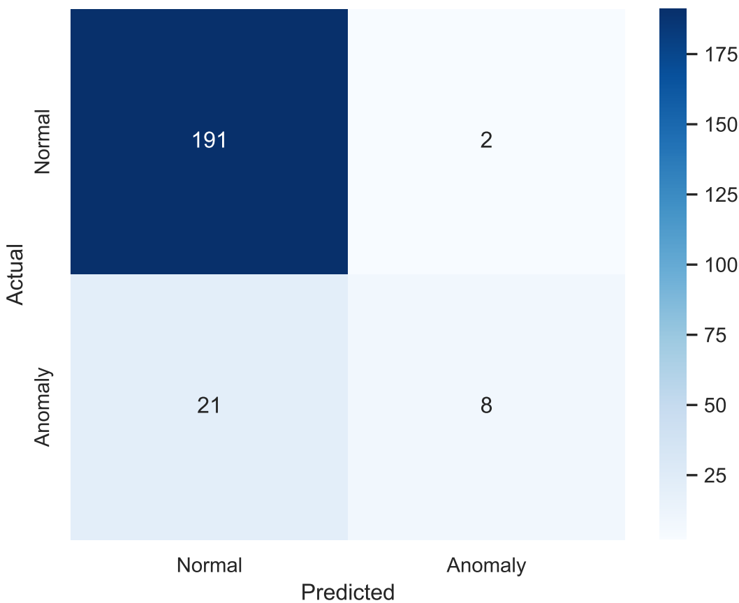
Confusion Matrix - GAN reconstruction score
