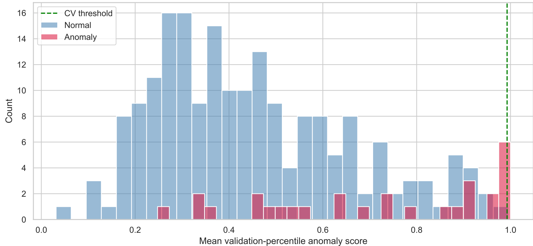
Ensemble anomaly score distribution on test window
