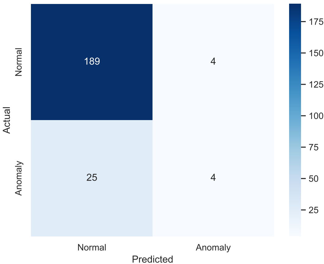
Confusion Matrix - GAN discriminator realism score
