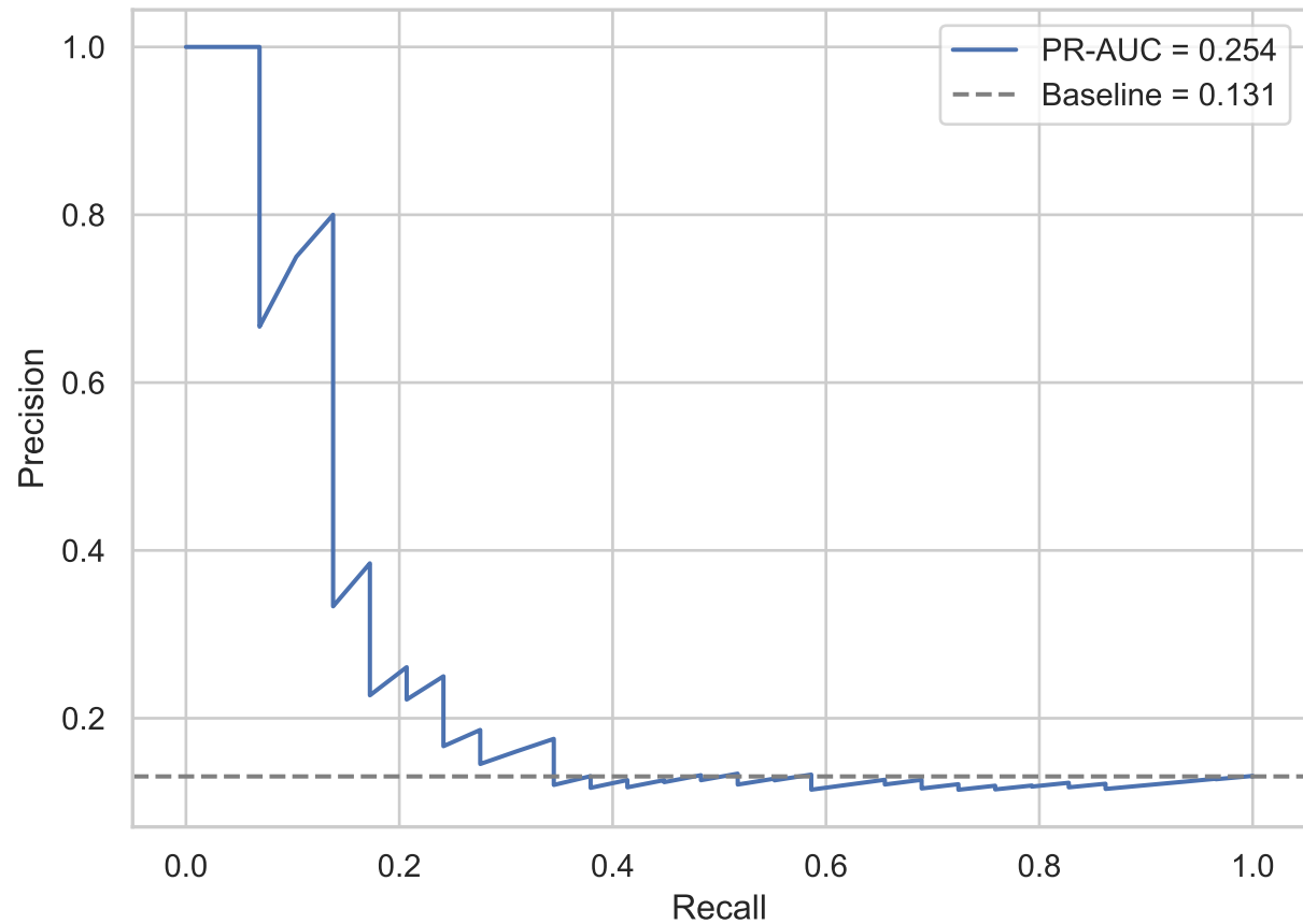
Precision-Recall - GAN discriminator realism score
