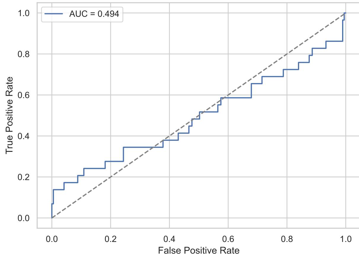
ROC - GAN discriminator realism score
