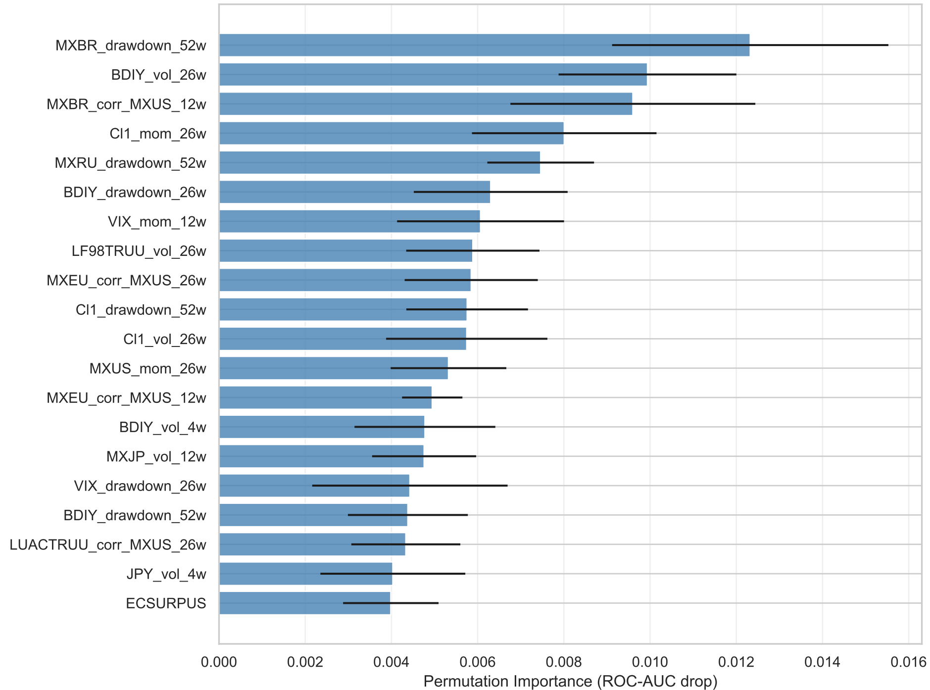
Top 20 features — Isolation Forest (importance = ROC-AUC decrease after permutation)
