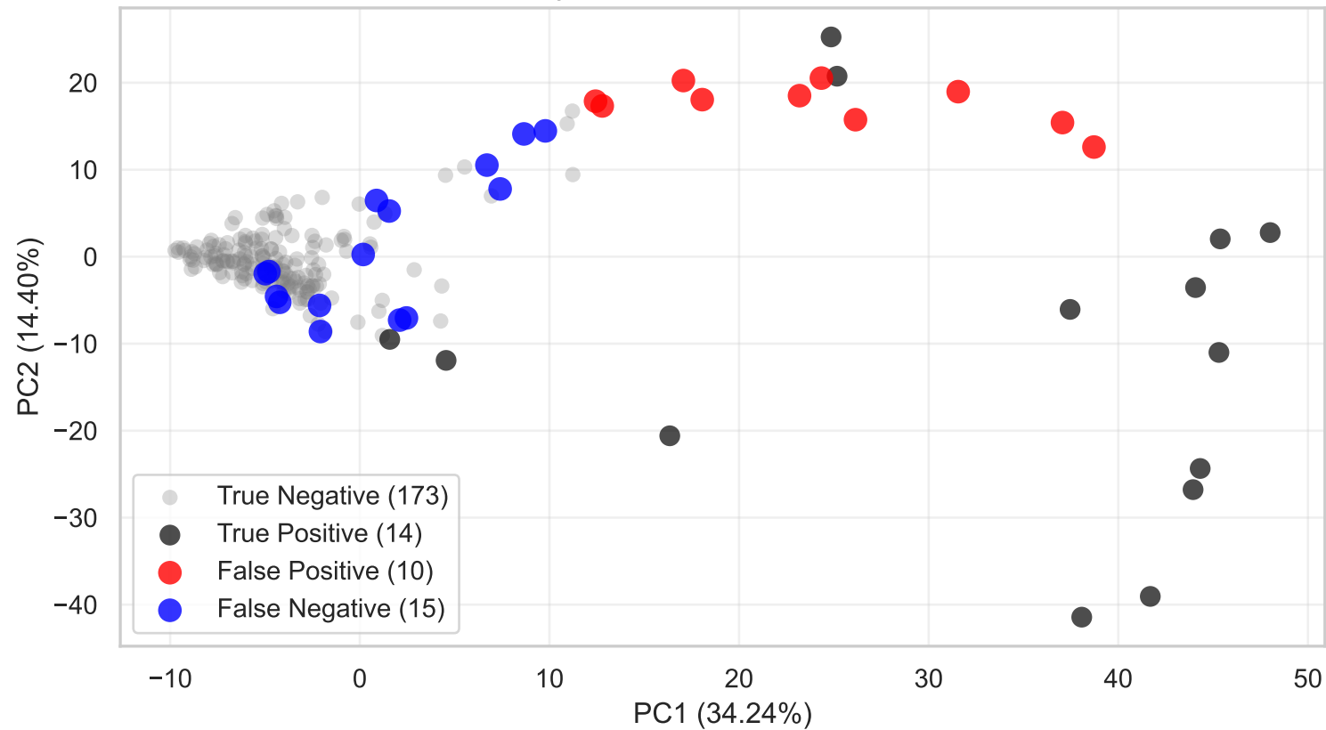
PCA projection — Test : F2-optimized threshold Explained variance: 48.64%
