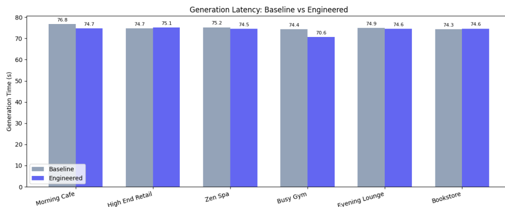
Figure 4: Generation time comparison: Baseline vs. Engineered latency for each vibe, averaging ~74 seconds per 30-second clip on A100 GPU.
